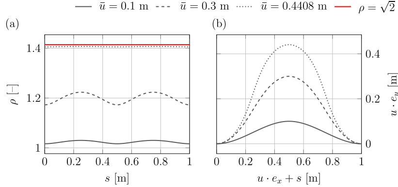
FIGURE 9. Three-point test. (a) Stretch \rho (b) Deformed configuration of macro-model.
