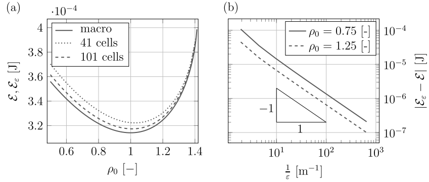
FIGURE 6. Semi-circle test. (a) Deformation energy of the micro-model (5), \mathcal{E}_\varepsilon , and the macro-model (24), \mathcal{E} (b) Discrete-continuum energy error on a log-log scale for different boundary conditions.
