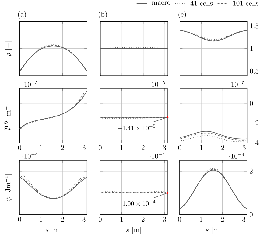
FIGURE 5. Semi-circle test. Stretch \rho , micro-strain \tilde{l}^{1D} and deformation energy density \psi of micro- and macro-model for (a) \rho_0 = 0.5 , (b) \rho_0 = 1 , and (c) \rho_0 = 1.405 .
