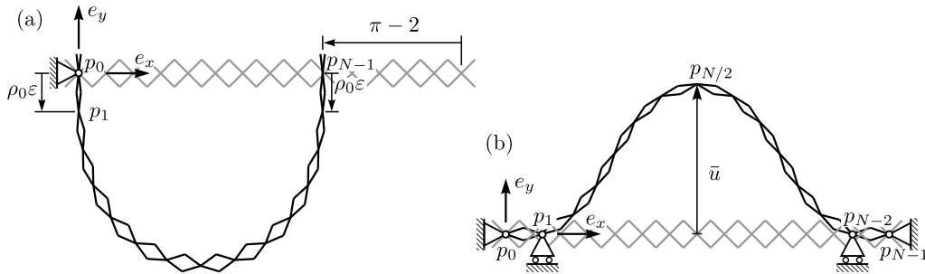
FIGURE 3. Boundary conditions, reference configuration (grey) and deformed configuration (black) for (a) Semi-circle test, \rho_0 = 1.405 (b) Three-point test, \bar{u} = 0.4 \text{ m} .
