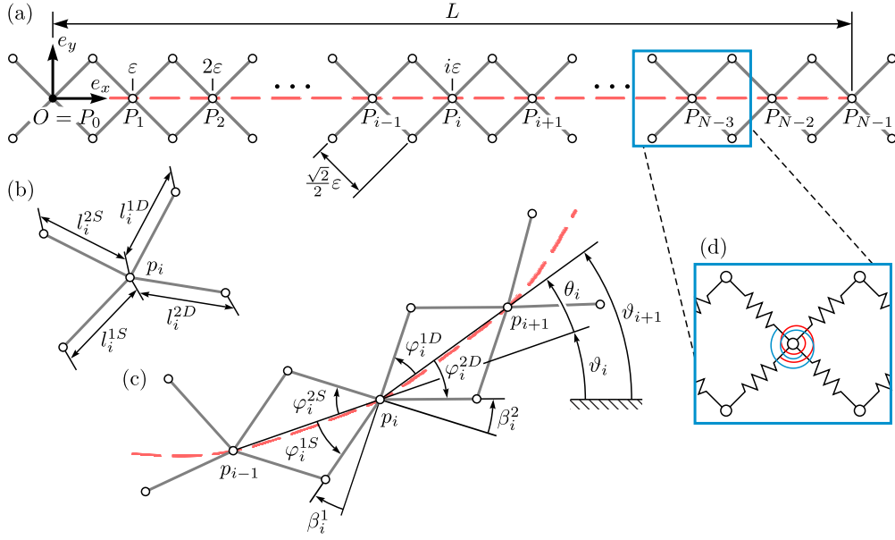
FIGURE 1. (a) Undeformed configuration (b) Generalized coordinates of i -th cell (c) Deformed configuration with redundant kinematic quantities (d) Force elements of a single cell.
