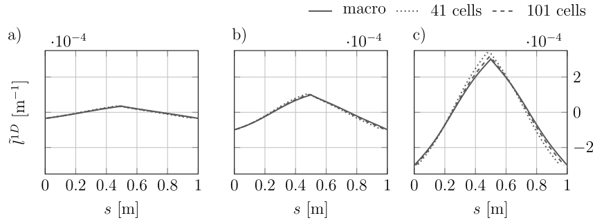
FIGURE 8. Three-point test. Micro-stretch \tilde{l}^{1D} of the micro- and macro-model for (a) \bar{u} = 0.1 m (b) \bar{u} = 0.25 m (c) \bar{u} = 0.4 m.
