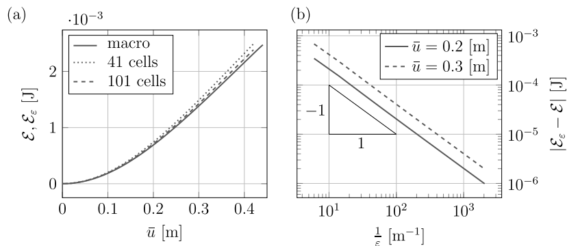
FIGURE 11. Three-point test. (a) Deformation energy of the micro-model (5), \mathcal{E}_\varepsilon , and the macro-model (24), \mathcal{E} (b) Discrete-continuum energy error on a log-log scale for different boundary conditions.
