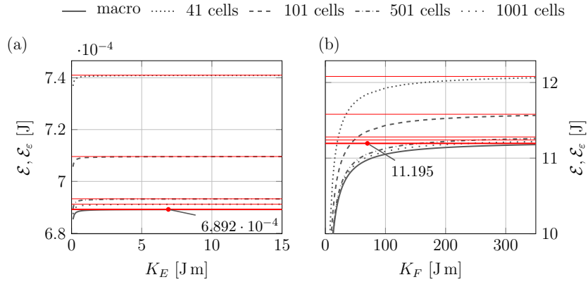
FIGURE 10. Three-point test. Deformation energy of the micro-model (5), \mathcal{E}_\varepsilon , and the macro-model (24), \mathcal{E} , for \bar{u} = 0.2 m. The red lines indicate the deformation energies for cases in which the kinematic constraints corresponding to (a) k_E \rightarrow \infty, K_E \rightarrow \infty or (b) k_F \rightarrow \infty, K_F \rightarrow \infty are enforced.
