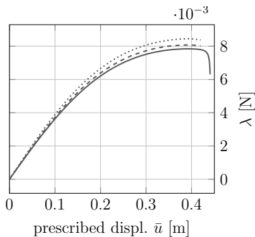
FIGURE 12. Three-point test. Plot of the Lagrange multiplier \lambda employed to enforce the constraint \chi(1/2) \cdot e_y = p_{N/2} \cdot e_y = \bar{u} (reaction force, rate of deformation energy with respect to \bar{u} according to Castigliano's theorem) vs \bar{u} for the continuum model (continuous line) and the discrete one (dotted line: 41 cells; dashed line: 101 cells). Newton-Raphson scheme has been employed for solving the micro-model.
