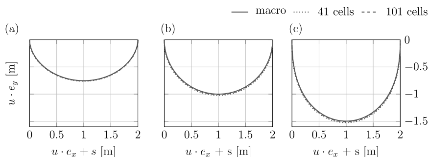
FIGURE 4. Semi-circle test. Deformed configurations of micro- and macro-model for (a) \rho_0 = 0.5 , (b) \rho_0 = 1 , and (c) \rho_0 = 1.405 .
