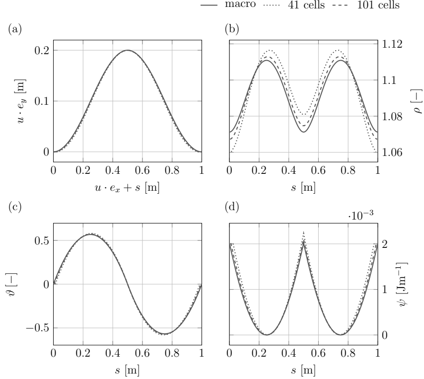
FIGURE 7. Three-point test. Micro- and macro model for \bar{u} = 0.2 m (a) Deformed configuration (b) Stretch \rho (c) Inclination angle \vartheta (d) Deformation energy density \psi .
